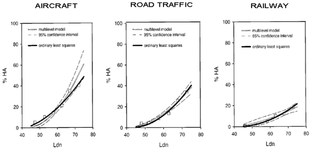
Figure B3. Miedema et al. [4] Community Annoyance prediction curves
