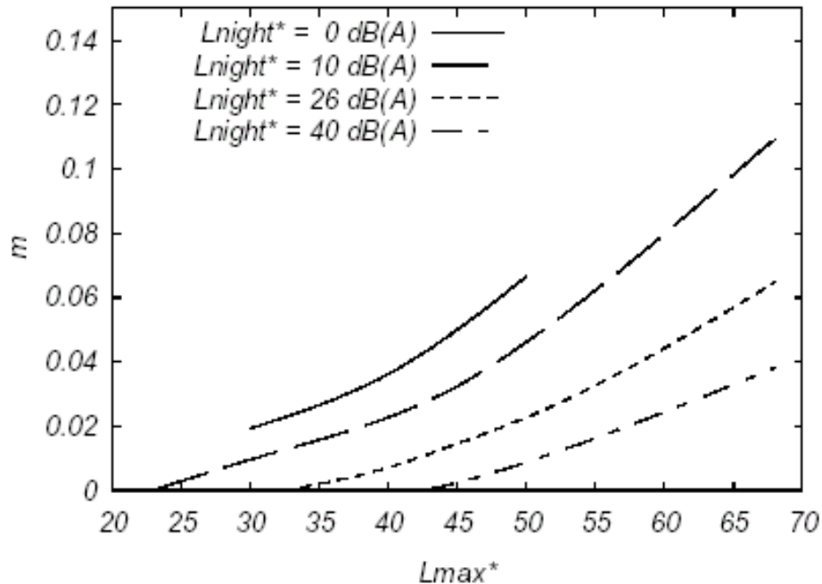
Figure B6. Probability of (aircraft) noise-induced motility ( m ) in the 15-s interval at which indoor maximum noise level occurs as a function of L_{max}^* , for various levels of long-term aircraft noise during sleep period ( L_{night}^* ) [8].
