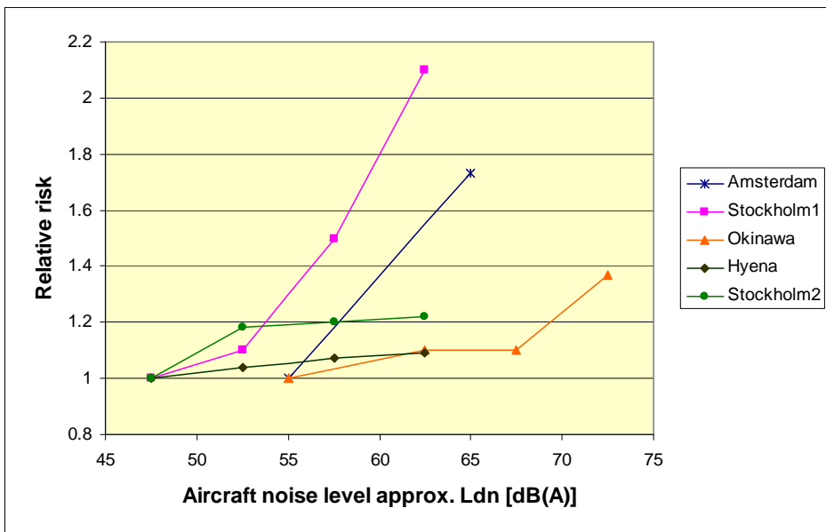
Figure B9. Association between aircraft noise level and the prevalence of hypertension [33].
