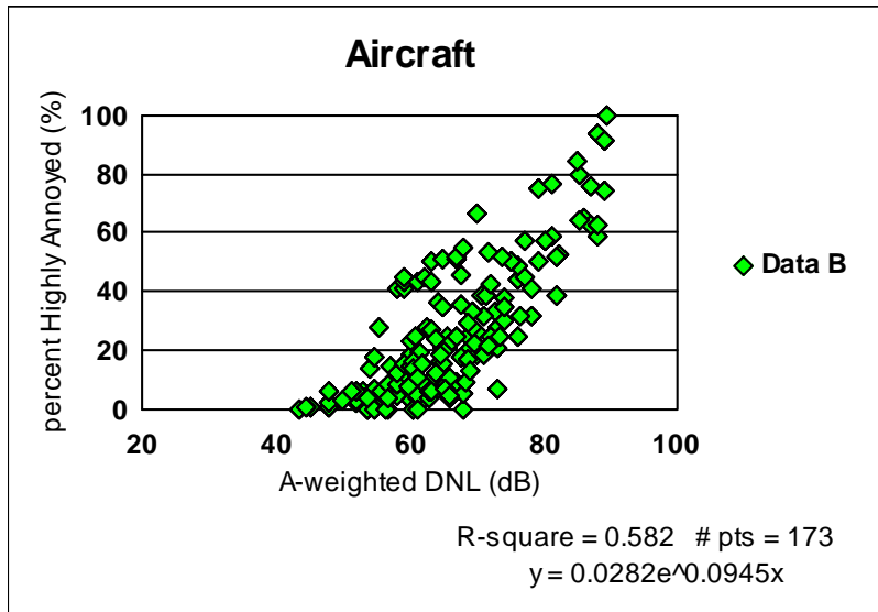
Figure 4.1. Data scatter for community annoyance in response to aircraft noise exposure (Finegold et al., 1994).
