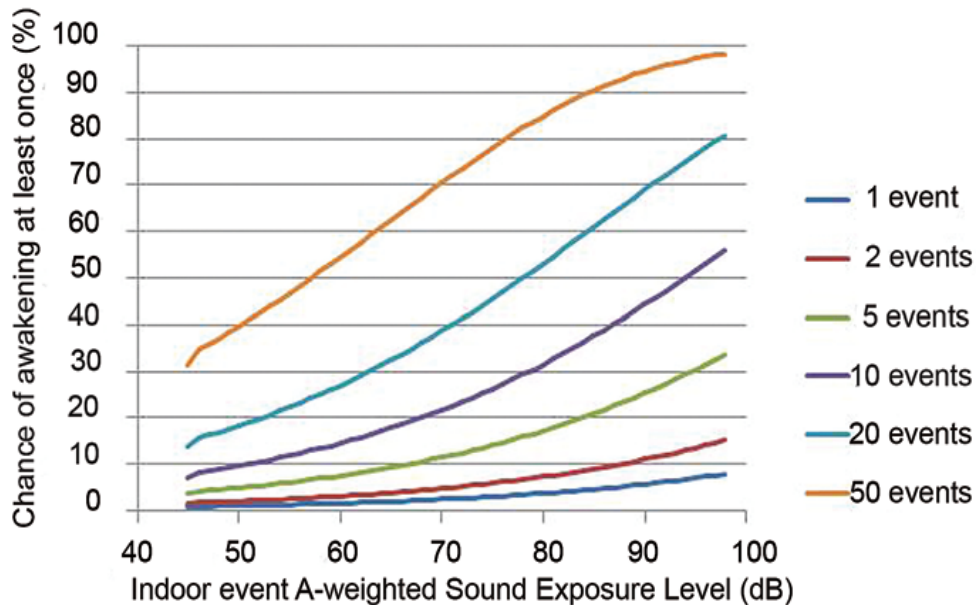
Figure B7. Chance of being awakened at least once versus event SEL for multiple, like noise events
