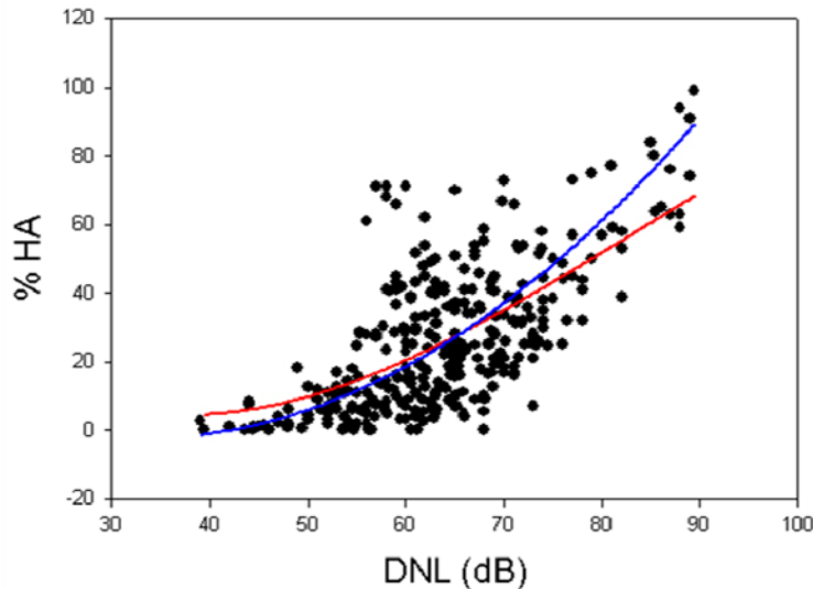
Figure B4. Scattergram of exposure-response relations, together with the (red) logistic regression curve for aircraft noise annoyance according to Fidell & Silvati [6], and the (blue) regression curve of Miedema & Vos [4] for aircraft noise. Note that the definition of “highly annoyed” is: 60-80 % of the length of the response scale.
