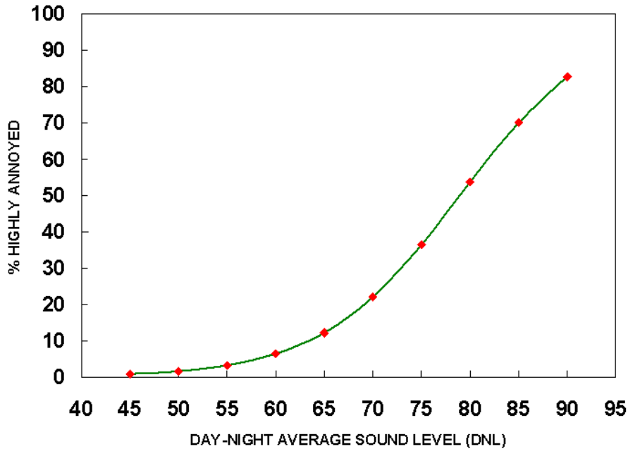
Figure B1. Community annoyance exposure-response curve from Finegold et al. [1]
