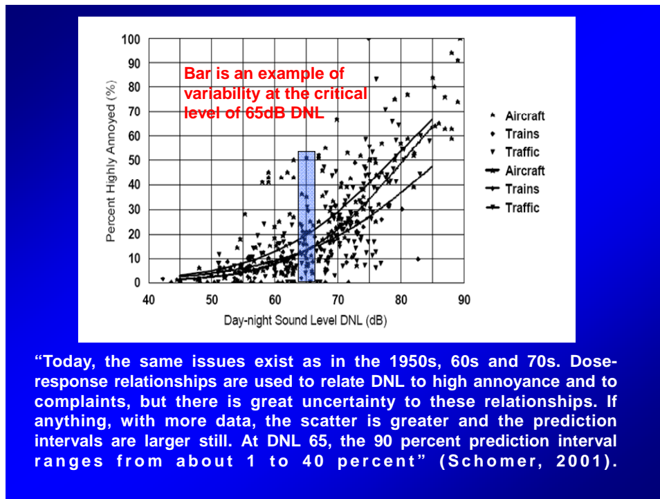
Figure 4.2. Community Annoyance - data variability at 65dB (A) DNL (modified from Schomer, 2001).
