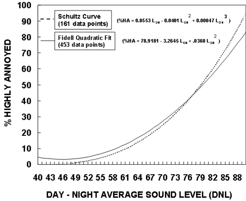
Figure B2. Community annoyance prediction curve from Fidell et al. [2], compared with original Schultz Curve [3]
