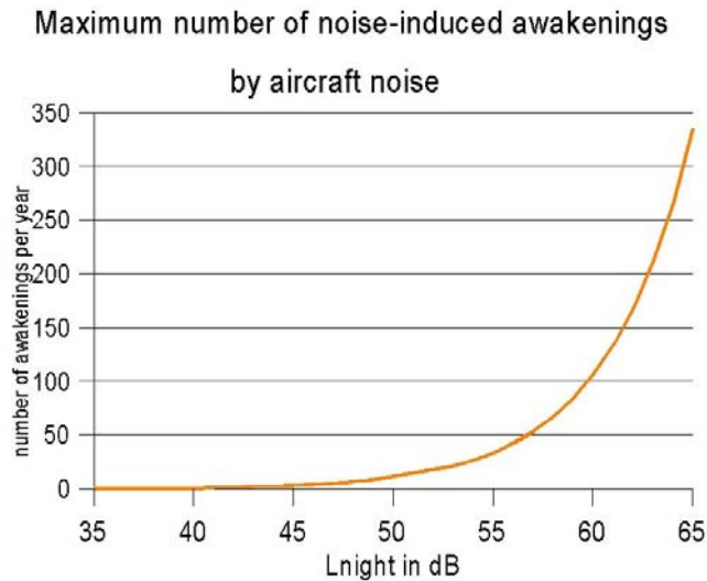
Figure B5. “Worst case” prediction of noise induced behavioral awakenings per year using L_{\text{night}} , converted from inside exposure data [12], based on data from Passchier-Vermeer [10]).
